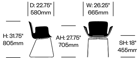
Side Chair with Sled Base
