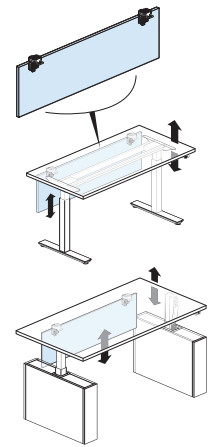
Adaptable Modesty Panel
