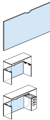
Full-Overlay Modesty Panel
