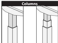
Columns Standard Range (Single Stage) Height Adjustment 27.1" (689mm) to 46.0" (1169mm) Extended Range (Dual Stage) Height Adjustment Low: 22.4" (569mm) to 48.3" (1227mm) High: 23.3" (592mm) to 50.0" (1270mm)
