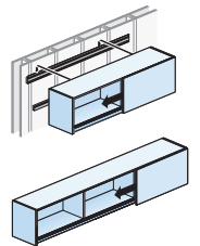
1H Overhead Storage Units with Sliding Door
