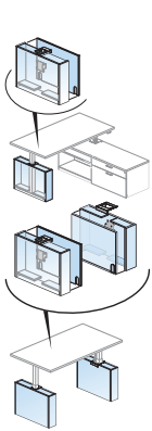
Shroud use with Height Adjustable T-Leg
