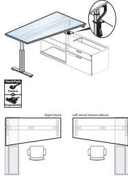
Height Adjustable Convergent Worktop Wedge Square T-Leg
